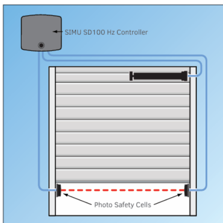
Photo Safety Cells
