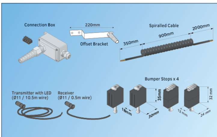
SIMU Safety Edge System Connection Kit
